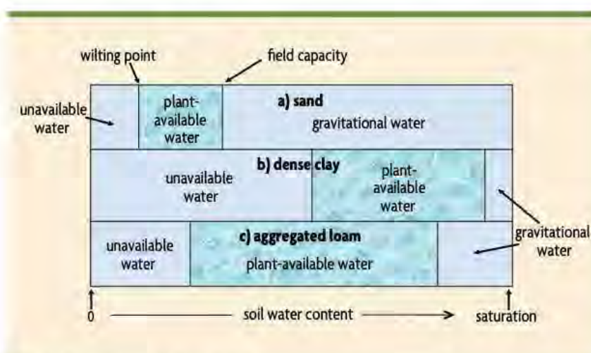
Figure 5.4. Water storage for three soils.
