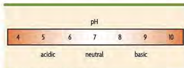
Figure 20.1. Soil pH and acid-base status.
