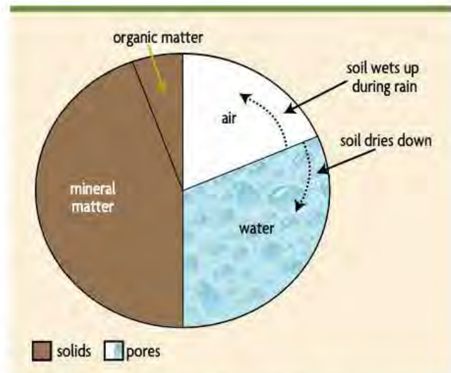
Figure 5.1. Distribution of solids and pores in soil.
