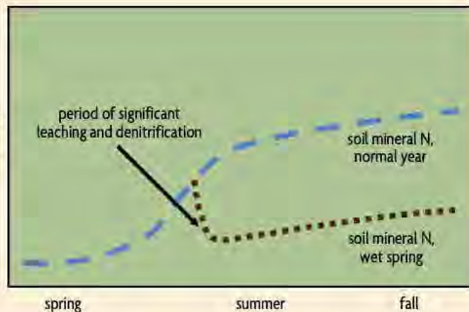
Figure 19.2. Available N in soil depends on recent weather. After increasing for a period, mineral N decreases during a wet spring because leaching and denitrification losses are greater than N being converted to mineral forms. More mineral N is available for plants when the spring is drier. (Gains and losses are greater when large amounts of organic applications, for example manure, are made.)
