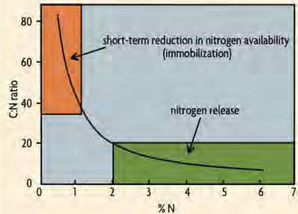
Figure 9.3. Nitrogen release and immobilization with changing nitrogen content. Based on data of Vigil and Kissel (1991).
