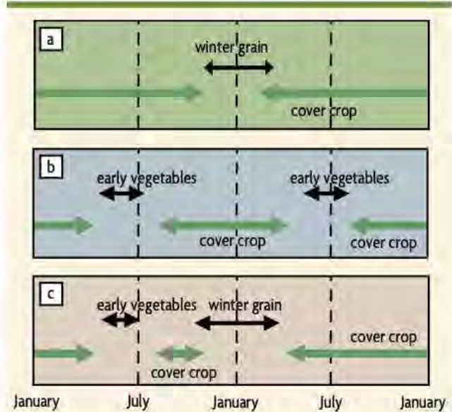
Figure 10.8. Timing cover crop growth for winter grain, early vegetable and vegetable-grain systems.
