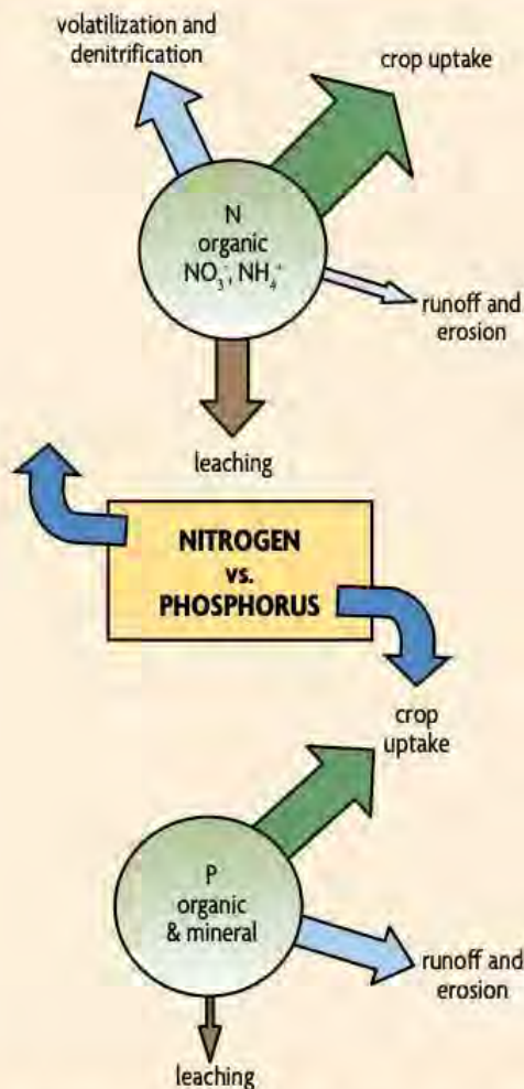
Figure 19.1. Different pathways for nitrogen and phosphorus losses from soils (relative amounts indicated by width of arrows). Based on an unpublished diagram by D. Beegle, Penn State University.
