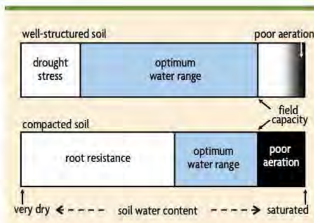
Figure 6.15. The optimum water range for crop growth for two different soils.
