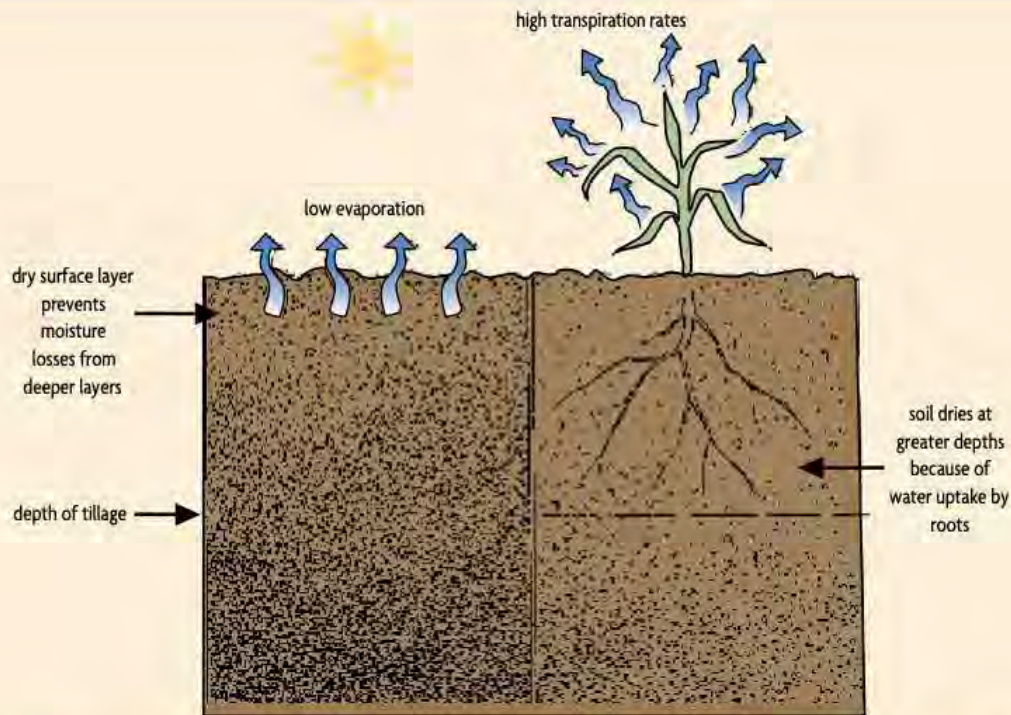
Figure 15.8. Cover crops enhance the drying of a clay soil. Without cover crops (left), evaporation losses are low after the surface dries. With cover crops (right), water is removed from deeper in the soil because of root uptake and transpiration from plant leaves, resulting in better tillage and traffic conditions.
