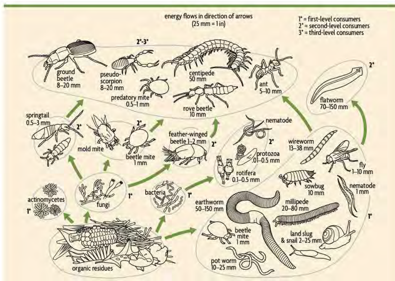
Figure 4.1. The soil food web. Modified from D.L. Dindal (1972). Illustration by Vic Kulihi.
