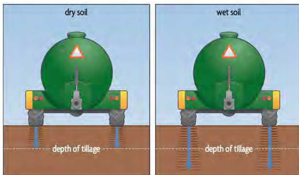
Figure 6.12. Forces of heavy tillage loads are transferred deep into the soil, especially when the soil is wet. Illustration by Vic Kulihin.
