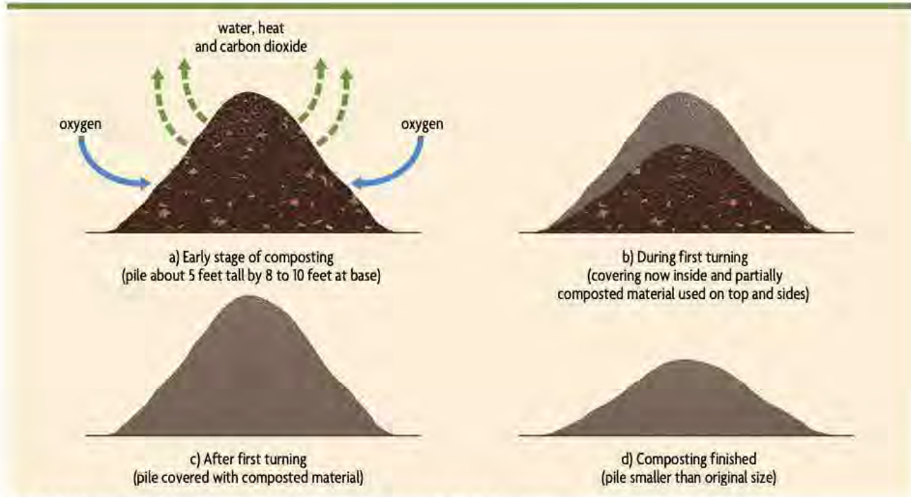
Figure 13.2. Compost pile dimensions and turning techniques. Illustration by Vic Kulihin.
