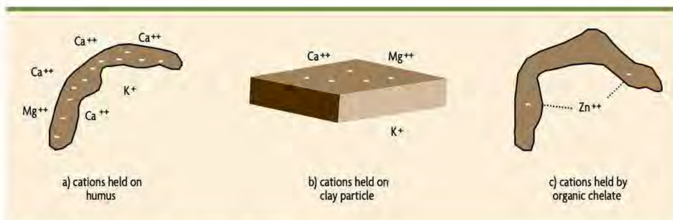
Figure 2.5. Cations held on negatively charged organic matter and clay.
