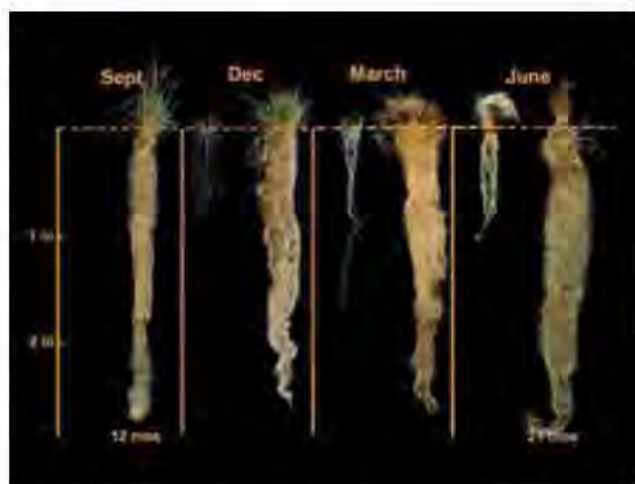
Figure 3.2. Root systems of annual wheat (at left in each panel) and wheatgrass, a perennial, at four times of the year. Approximately 25–40% of the wheatgrass root system dies back each year, adding considerable amounts of organic matter, and then grows back again. Compared to annual wheat, it has a longer growing season and has much more growth both above ground and below ground. Wheatgrass was 12 and 21 months old when the first and last photos were taken. Photo by the Land Institute.
