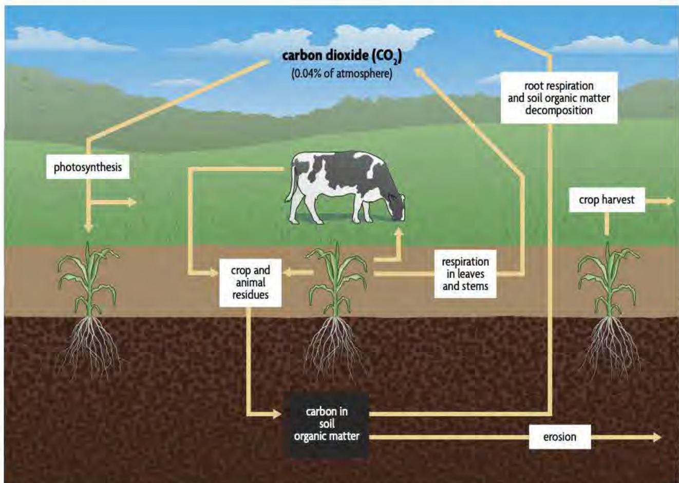
Figure 2.8. The role of soil organic matter in the carbon cycle. Illustration by Vic Kulihi.
