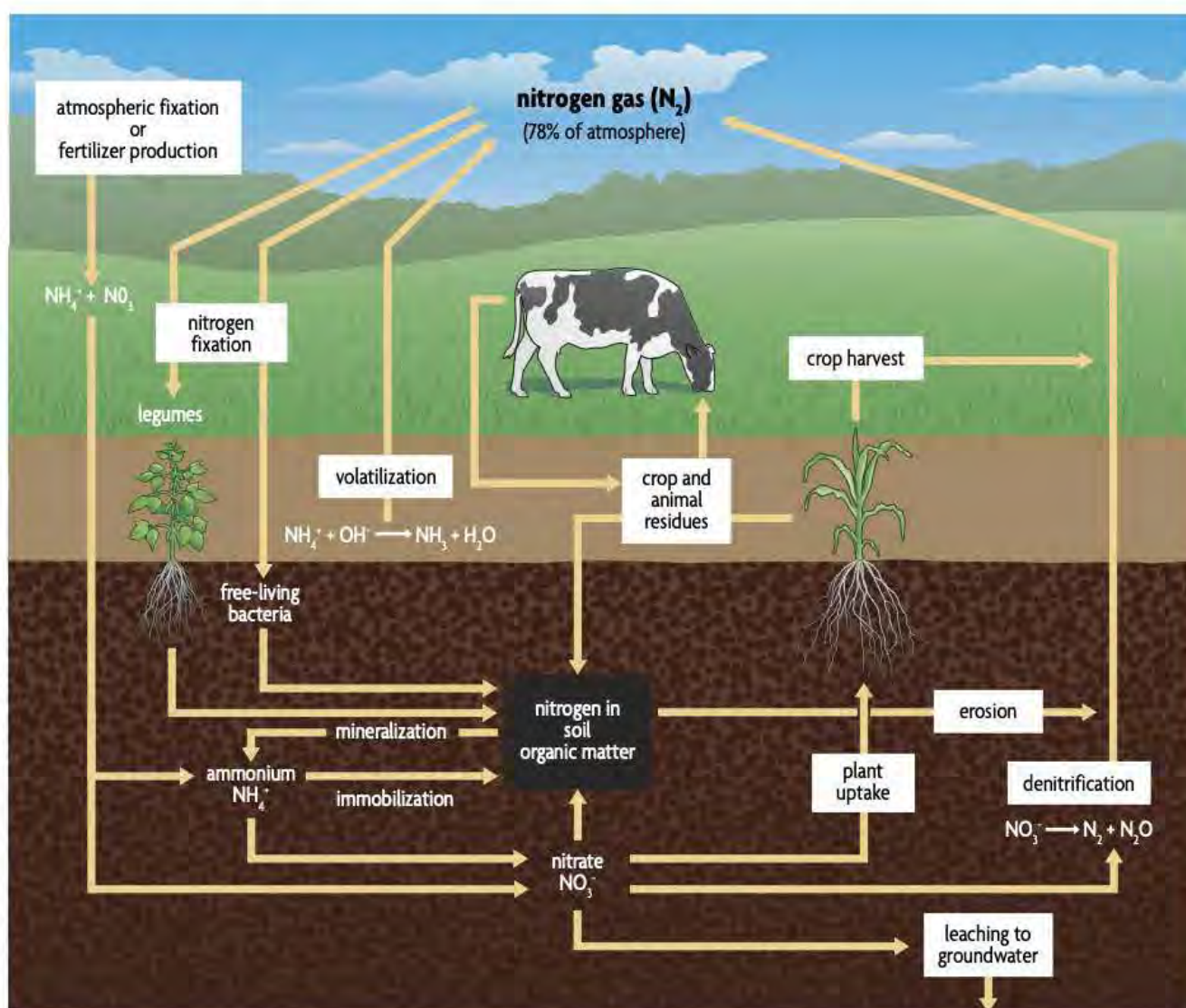
Figure 2.9. The role of organic matter in the nitrogen cycle. Illustration by Vic Kulihin.
