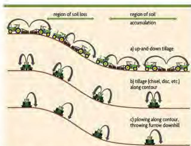
Figure 6.7. Three causes of erosion resulting from tilling soils on slopes. Illustration by Vic Kulihin.
