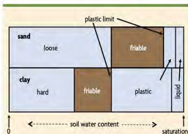
Figure 6.9. Soil consistency states for a sand soil and for a clay soil (friable soil is best for tillage).
