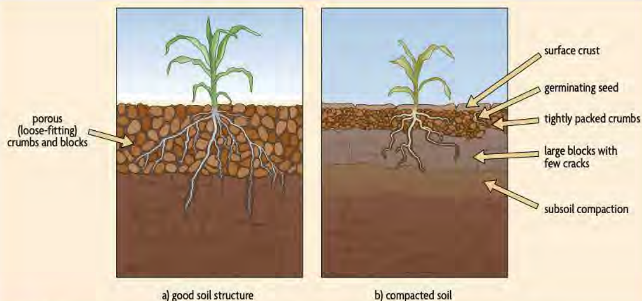
Figure 6.8. Plants growing in (a) soil with good tilth and (b) soil with all three types of compaction. Illustration by Vic Kulihin.
